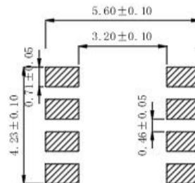
建议焊盘尺寸图 Recommended Soldering Pattern
