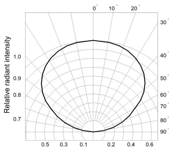
Fig.6 Radiation diagram
