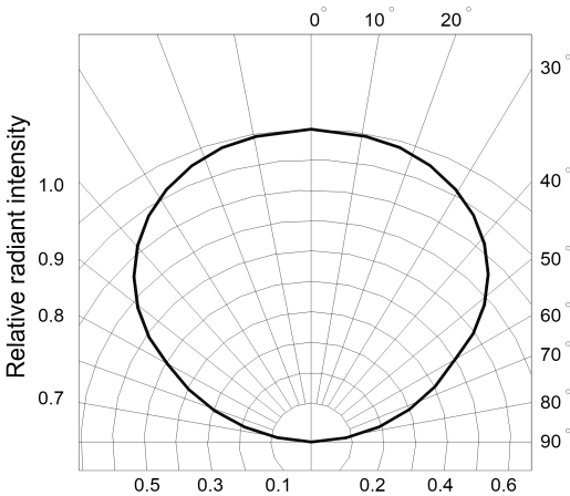
Fig.6 Radiation diagram
